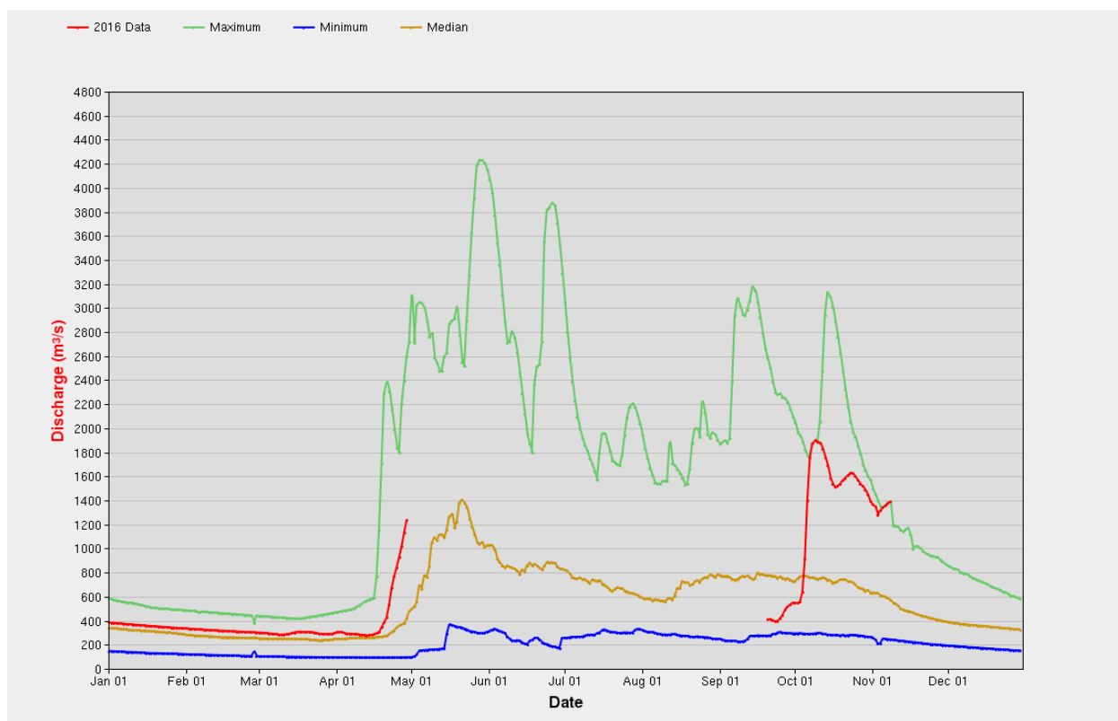
Figure 6-15: Historical daily discharge graph for the Hayes River (04AB001) Hydrometric Station (1973 to 2016)
