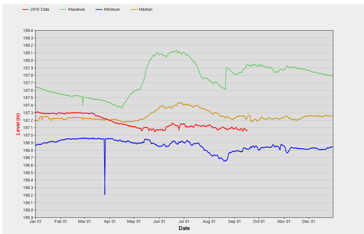
Figure 6-13: Historical daily water levels for Back Lake (04AA003) Hydrometric Station (1970 to 2016)
