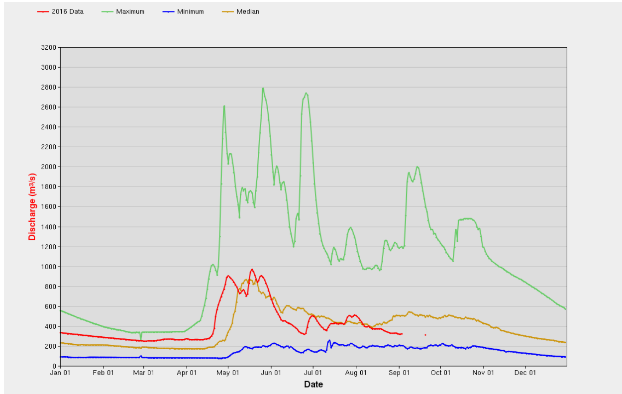
Figure 6-14: Historical daily discharge graph for the God's River at Confluence with Hayes River (04AD002) Hydrometric Station (1968 to 2016)
